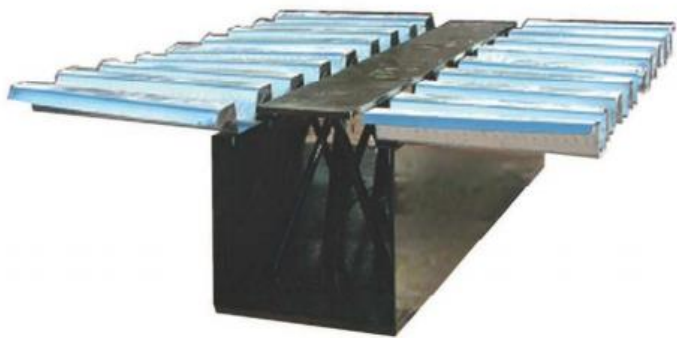
HEC TRAVE EMERGENTE
